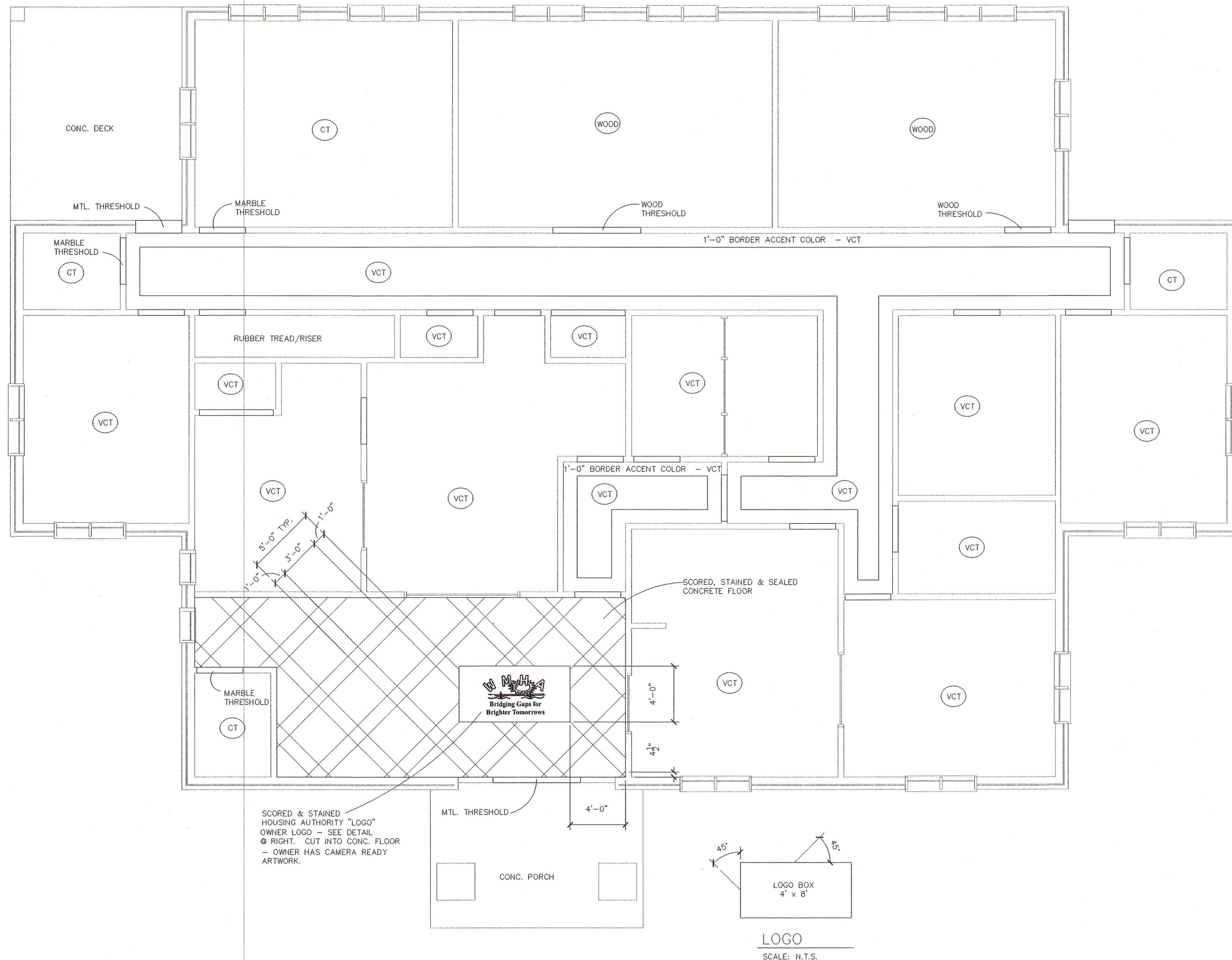
PLAN NORTH 1 A1-3 SCALE: 1/4" = 1'-0" FIRST FLOOR PATTERN PLAN
